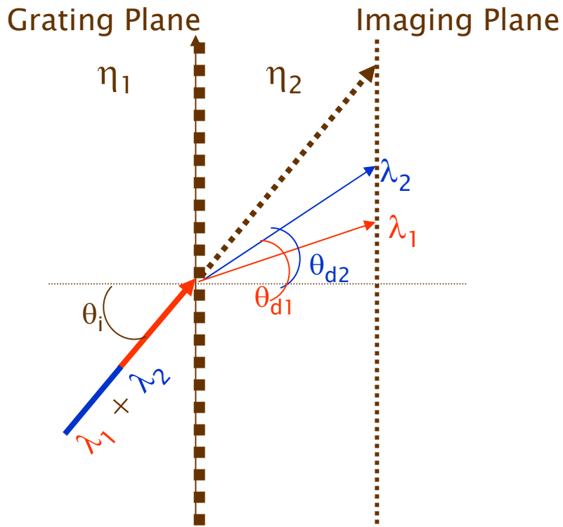
Transmission Grating
